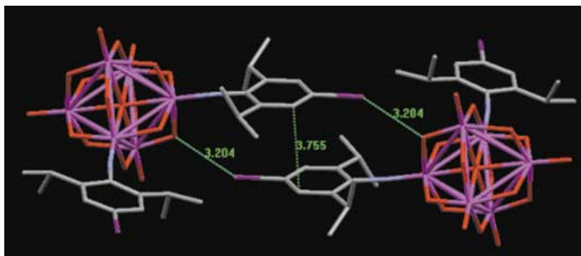
Figure 3. Dimer formation of the anions 2c in the lattice of (\text{Bu}_4\text{N})_2\text{2c} . Highlighted numbers indicate the interatomic distances [Å].
